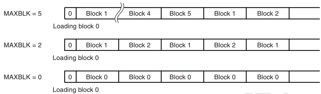
Figure 5-5. Examples for Different MAXBLK Settings
