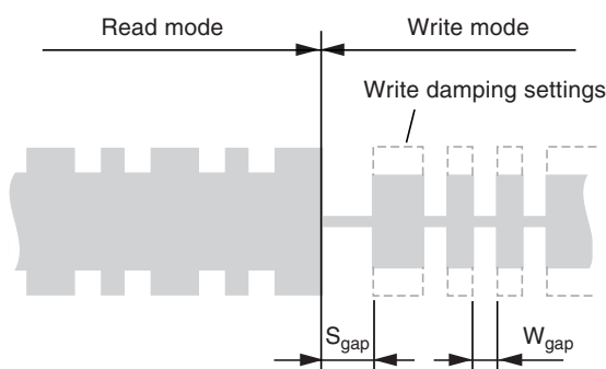
Figure 5-9. Start of Reader-to-tag Communication
