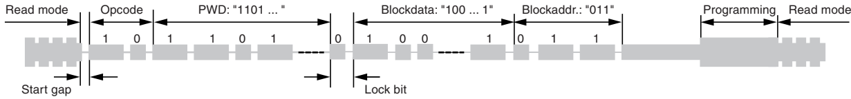
Figure 5-18. Protected Write Sequence Example
