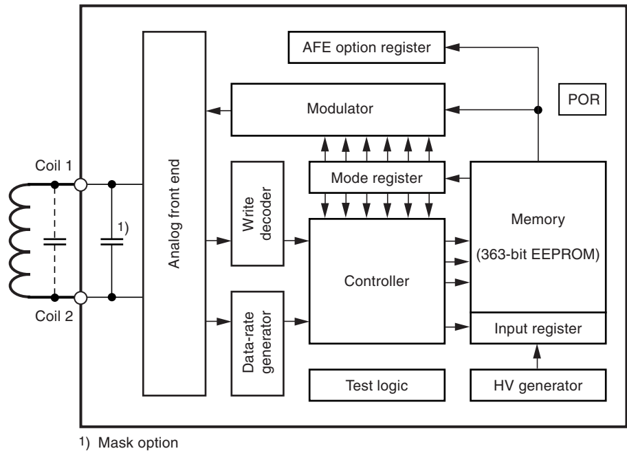
Figure 4-1. Block Diagram
